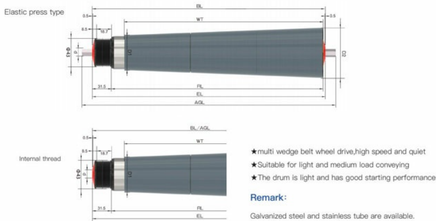
Plastic Poly-V Belt Conveyor Roller Tapered Drum For Curved Conveyor
